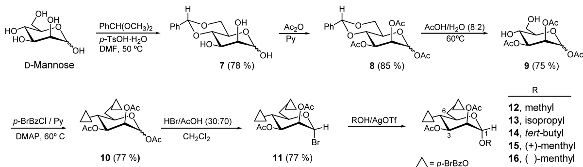
Scheme 2. Synthesis of the alkyl 2,3-bis- O -acetyl-4,6-bis- O -( p -bromobenzoyl)- \alpha -D-mannopyranosides.
