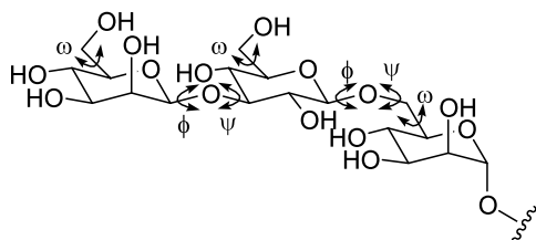
Figure 1. Torsion angles \phi and \psi around the glycosidic linkages, and torsion angles \omega around the C5–C6 bonds.
