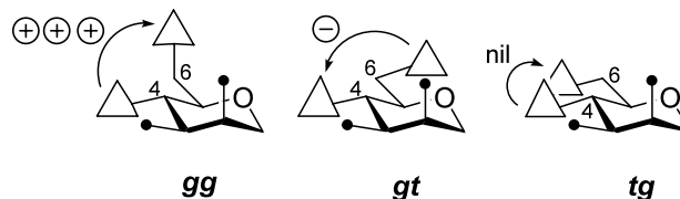
Figure 6. 4/6 Pairwise interaction for the mannopyranosyl system in each of the three stable rotamers ( gg , gt , and tg ).
