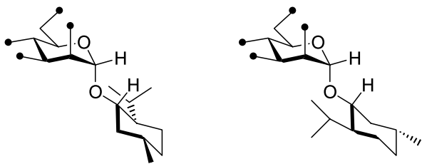
Figure 4. Structures of (1 S ,2 R ,5 S )-(+)- and (1 R ,2 S ,5 R )-(–)-menthyl \alpha -D-mannopyranosides, left and right, respectively.
