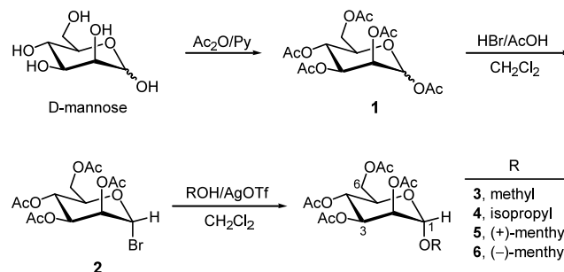
Scheme 1. Synthesis of the alkyl 2,3,4,6-tetrakis- O -acetyl- \alpha -D-mannopyranosides.
