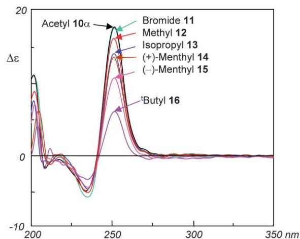
Figure 5. CD spectra comparison of the 1-acetyl 10α , the bromide 11 , as well as the model alkyl mannopyranosides 12–16 (CH 3 CN).
