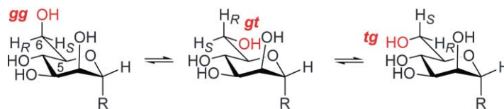
Figure 2. Molecular structure of an \alpha -D-mannopyranoside in its three main rotamers, the gg ( \omega = -60^\circ ), gt ( \omega = 60^\circ ), and tg ( \omega = 180^\circ ) rotamers around the C5–C6 bond.
