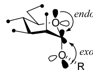
Figure 3. Illustration of the molecular orbitals involved in the exo - and endo -anomeric effects.
